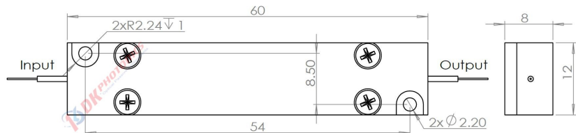
Dimension for <30W
