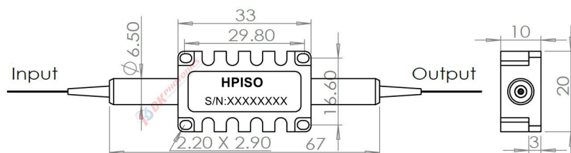
Dimension for 50W
